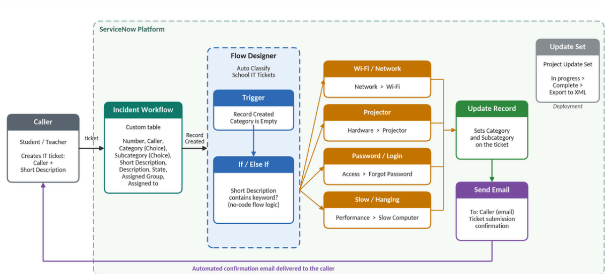
Figure 1: Architecture and data flow of the Auto Ticket Classification solution
